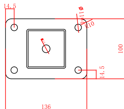
65x65-Flanged
