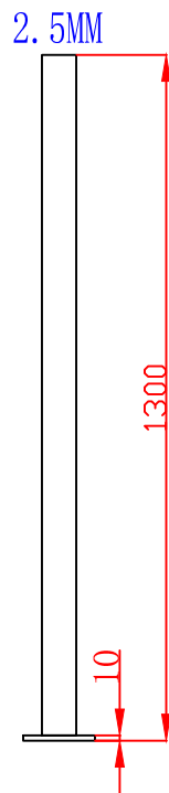
65X65-1300MM
