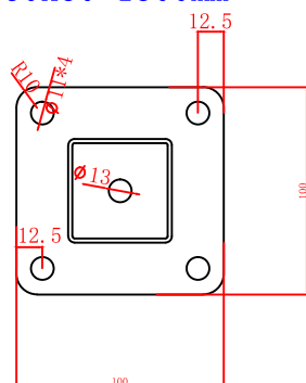
50x50-Flanged
